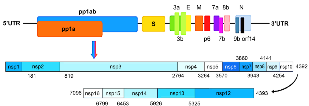
Fig. 3. ORF's of the genome of HB01 strain of SARS-CoV-2 (previously called 2019-nCoV) are shown. Structural proteins are encoded at the 3' terminus and non-structural at the 5' terminus (Modified from [40]).
