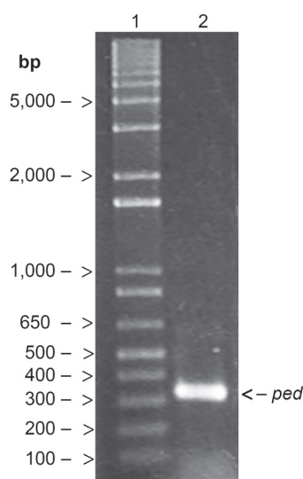
Fig. 3. DNA fragments obtained after PCR with plasmid DNA from P. acidilactici QC38 using Pediocin PA1-specific primers.
