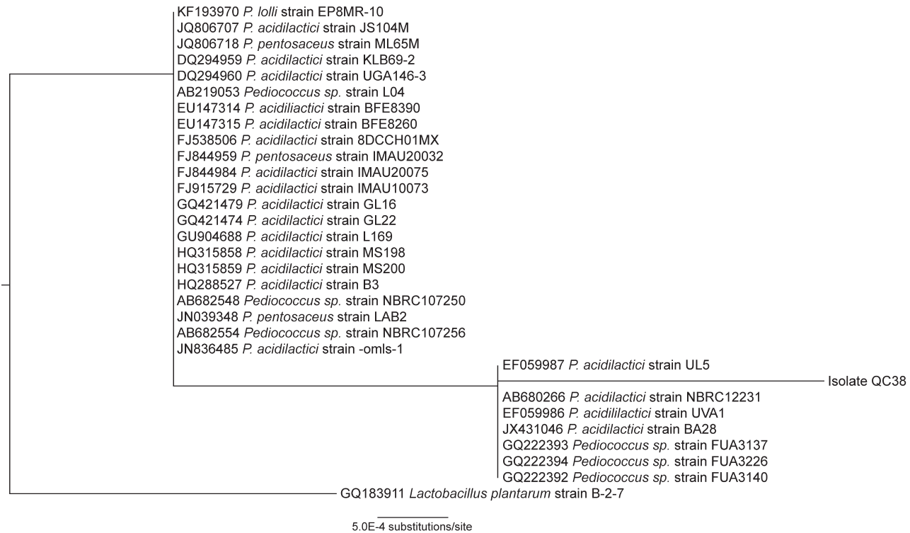
Fig. 1. ML tree reconstruction based on 516 bp from 16S Pediococcus species.
